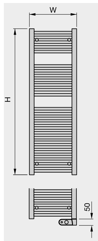
Adjustable thermostatic controller
