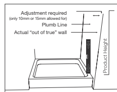
Diagram 3 Out of True Wall
