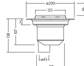
Quad Gravity Drain Tiled Insert 14mm - Vertical Outlet
