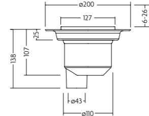
Quad Gravity Drain Slot - Vertical Outlet
