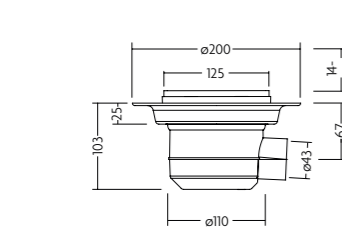
Quad Gravity Drain Tiled Insert 14mm - Horizontal Outlet
