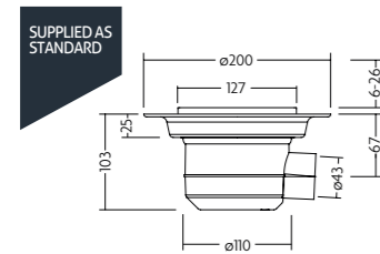
Quad Gravity Drain Slot - Horizontal Outlet
