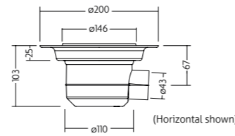
Vinyl Floor Gully - Horizontal Outlet
