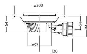
Tiled Drain Slim+ Horizontal Slot
